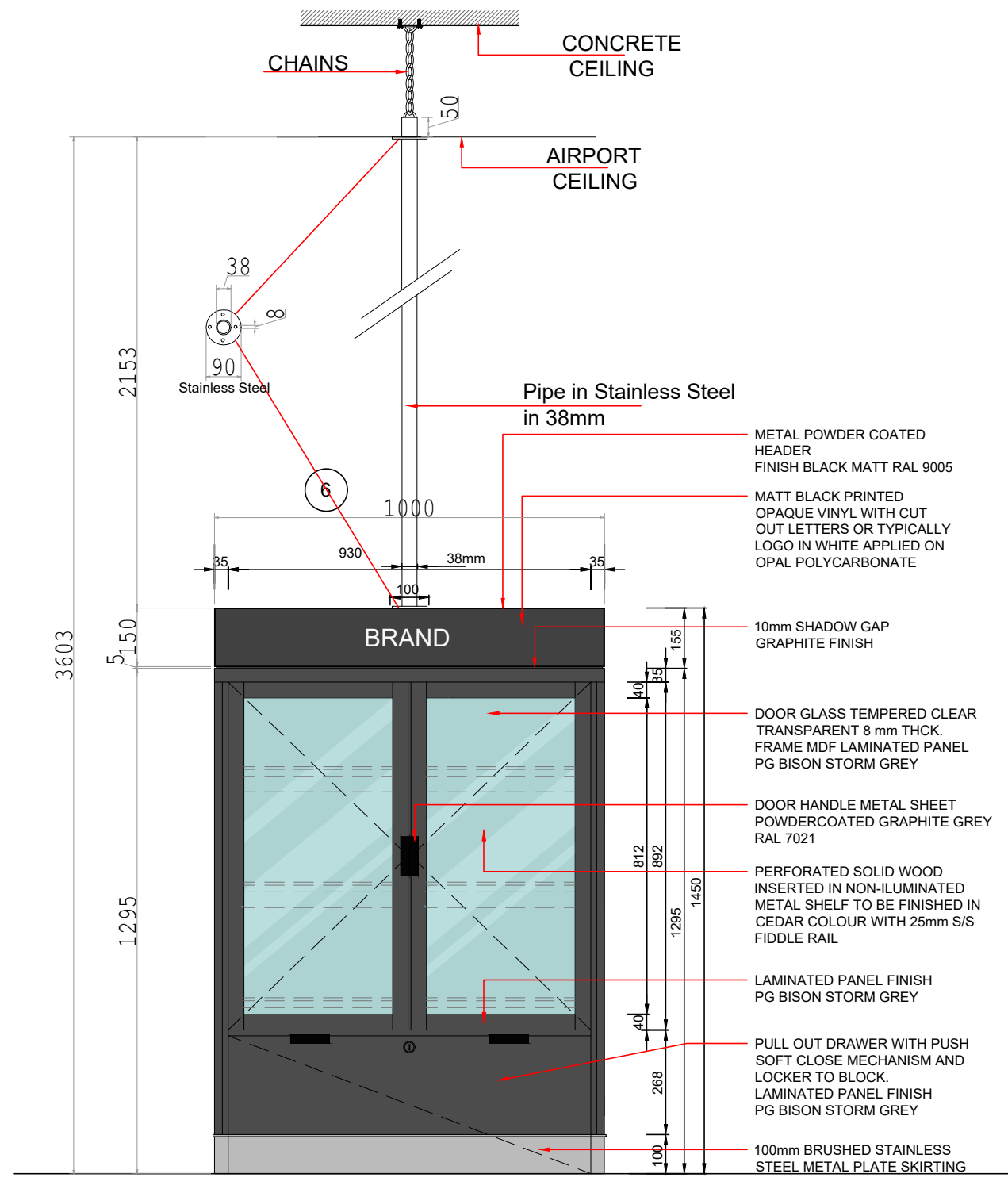
2 FRONT ELEVATION
